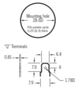
Panel mounting
