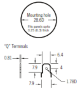
Panel mounting
